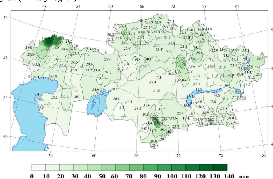
Figure 3.5 – Daily maximum precipitation in 2023 ( Rx1day index )
