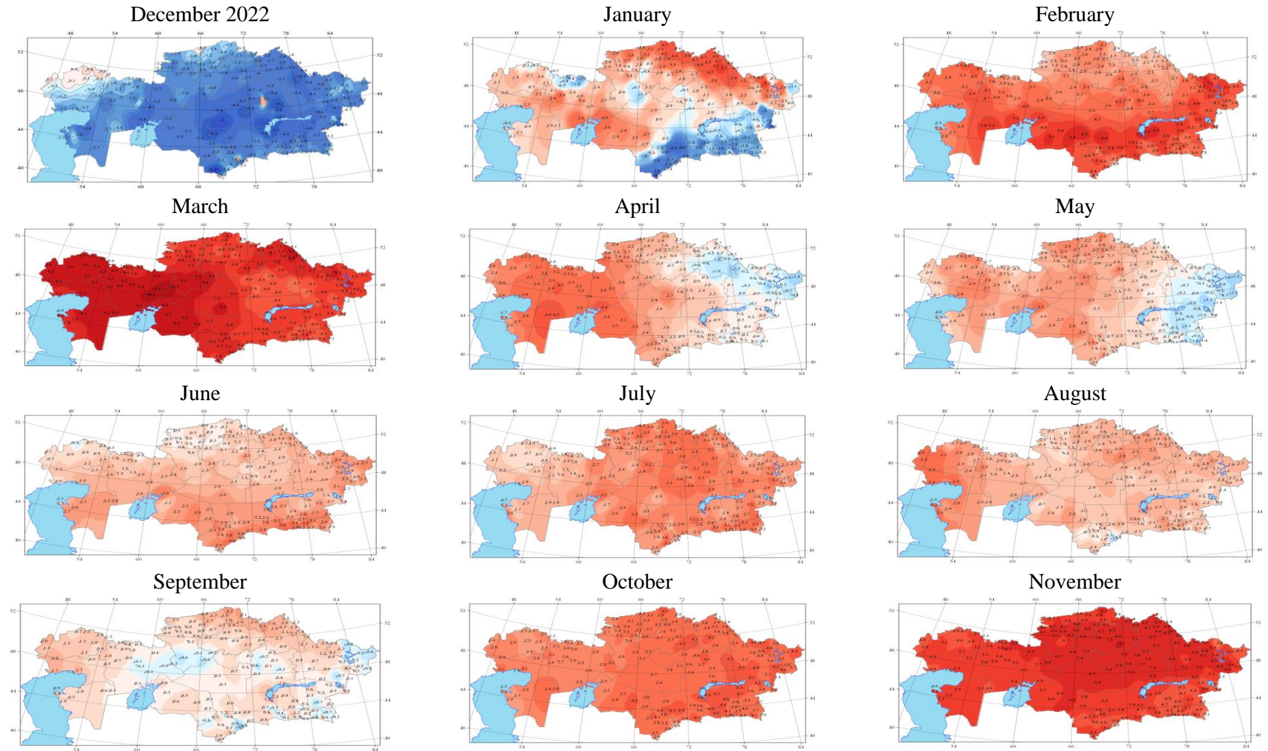
Figure 2.5 – Spatial distribution of the anomaly of the average monthly air temperature ( ^{\circ}\text{C} ) in 2023, calculated relative to the base period of 1961-1990.
