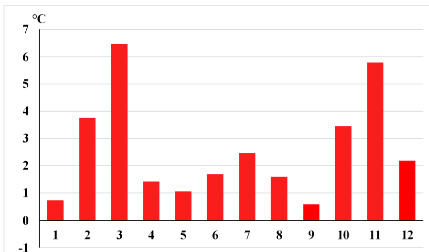
Figure 2.3 – Average monthly air temperature anomalies averaged over the territory of Kazakhstan in 2023, calculated relative to the average for the period 1961-1990.
