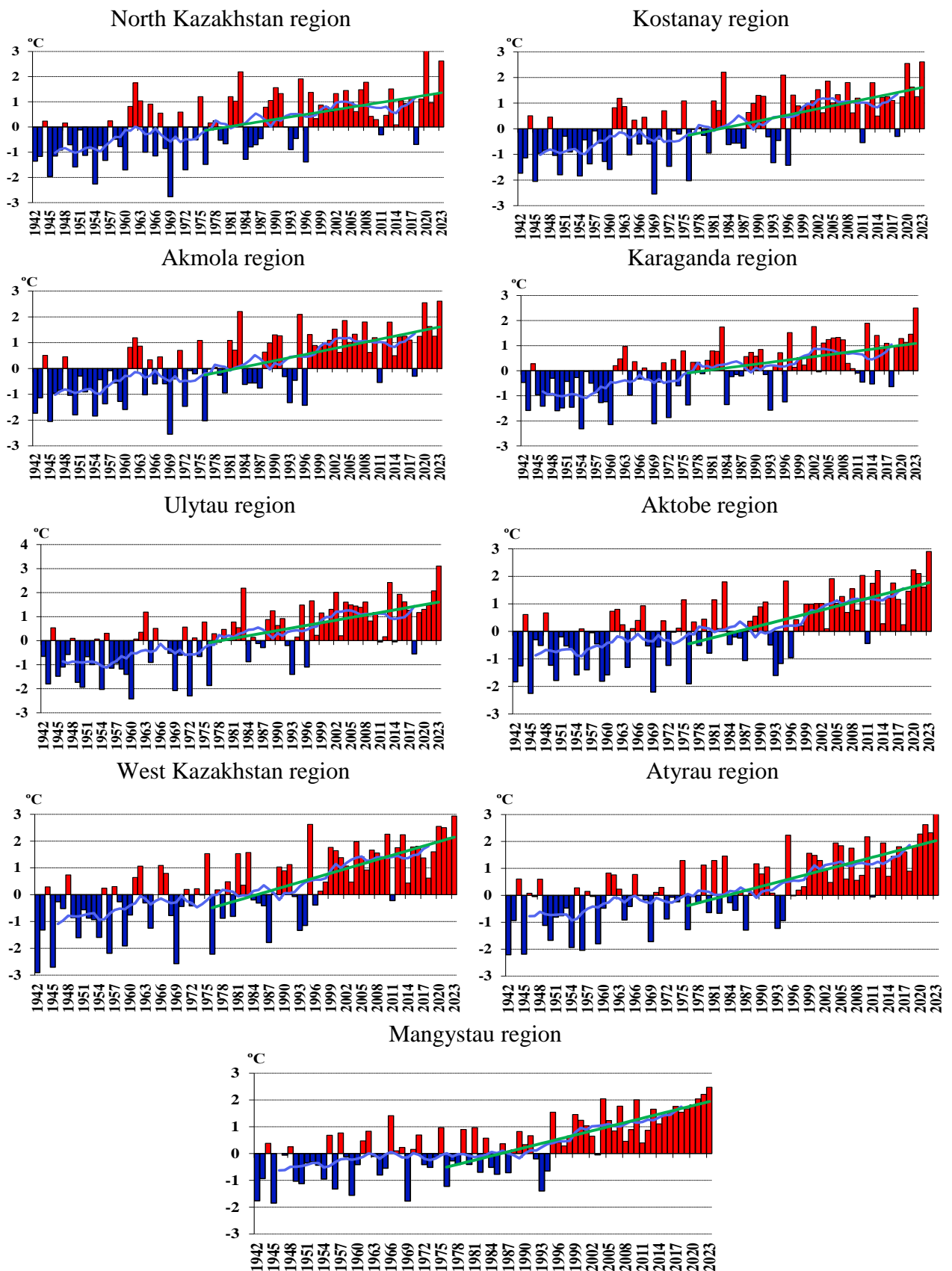
Figure 2.15 – Time series of anomalies of annual air temperatures (°C) averaged over the regions of Kazakhstan for the period 1941-2023. The anomalies are calculated relative to the base period of 1961-1990. The linear trend for the period 1976-2023 is highlighted in green. The smoothed curve is obtained by an 11-year moving average. Sheet 2
