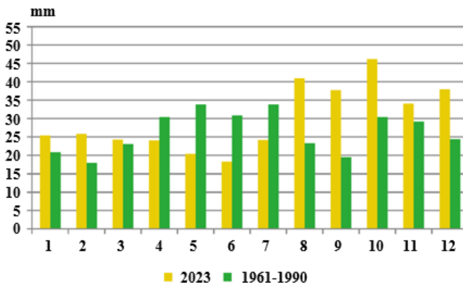
Figure 3.2 – Territory-averaged monthly precipitation sums in Kazakhstan in 2023 and their norms, calculated for the period 1961–1990
