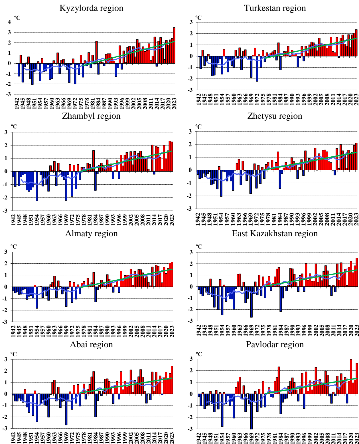
Figure 2.15 – Time series of anomalies of annual air temperatures (°C) averaged across the regions of Kazakhstan for the period 1941-2023. The anomalies are calculated relative to the base period of 1961-1990. The linear trend for the period 1976-2023 is highlighted in green. The smoothed curve is obtained by an 11-year moving average. Sheet 1
