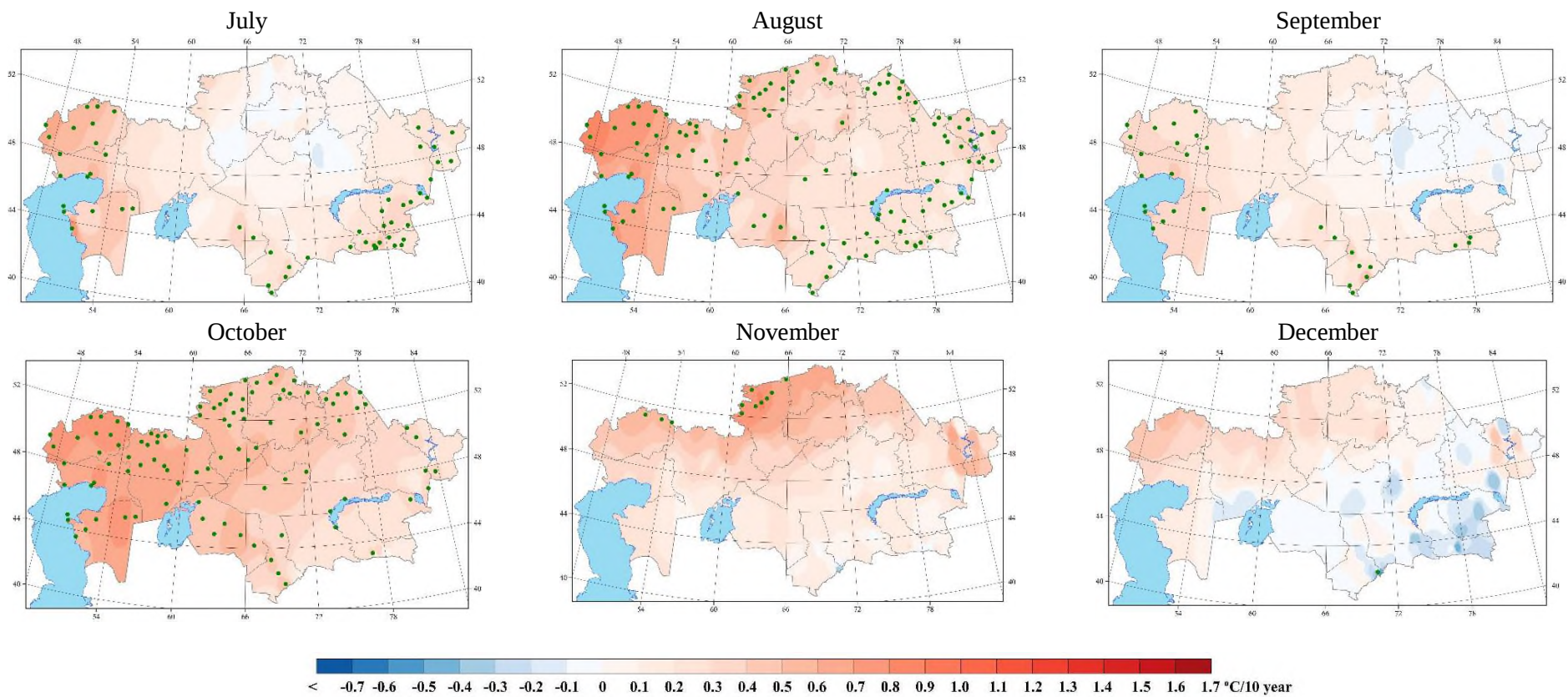
Figure 2.17 – Spatial distribution of values of the linear trend coefficient of the mean monthly surface air temperature ( ^{\circ}\text{C}/10 years) calculated from the observation data for the period 1976–2024. Sheet 2
