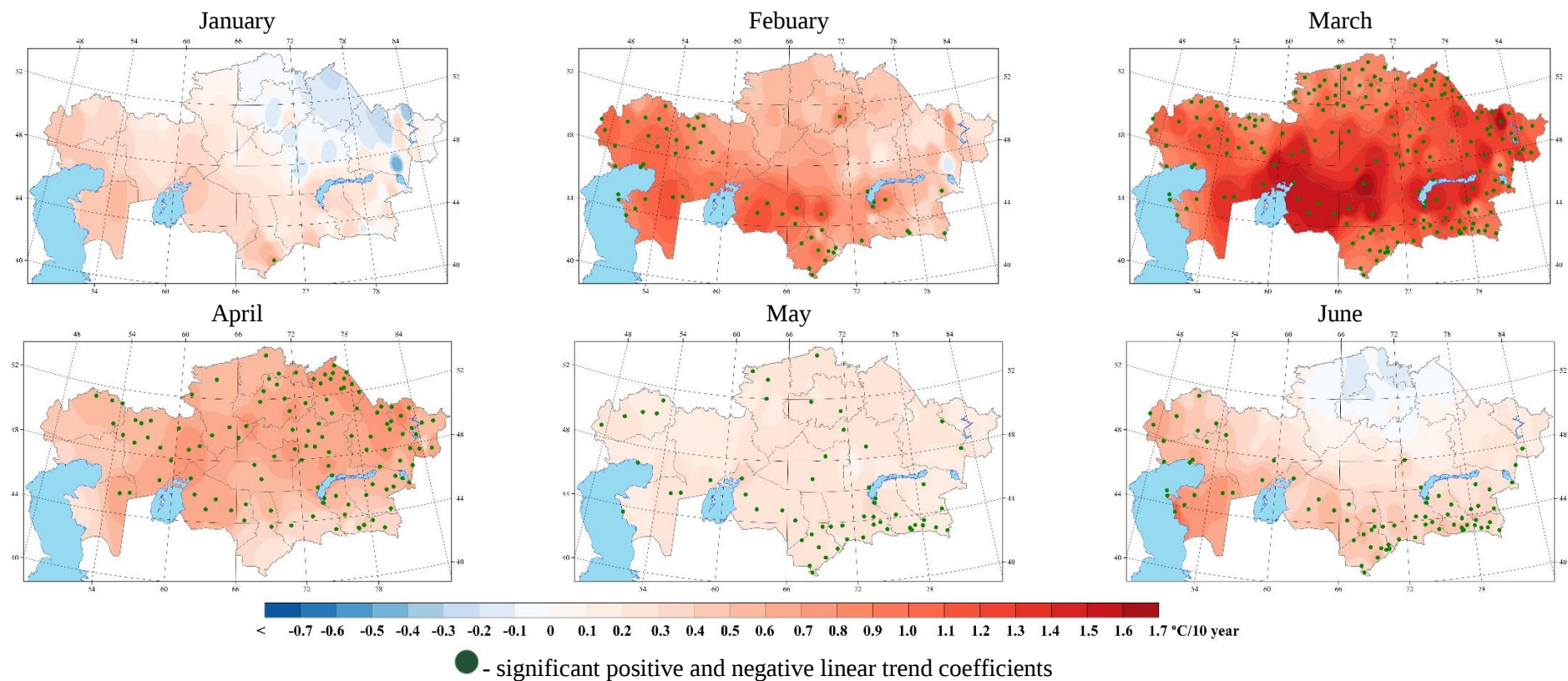
Figure 2.17 – Spatial distribution of values of the linear trend coefficient of the mean monthly surface air temperature (°C/10 years) calculated from the observation data for the period 1976–2024. Sheet 1
