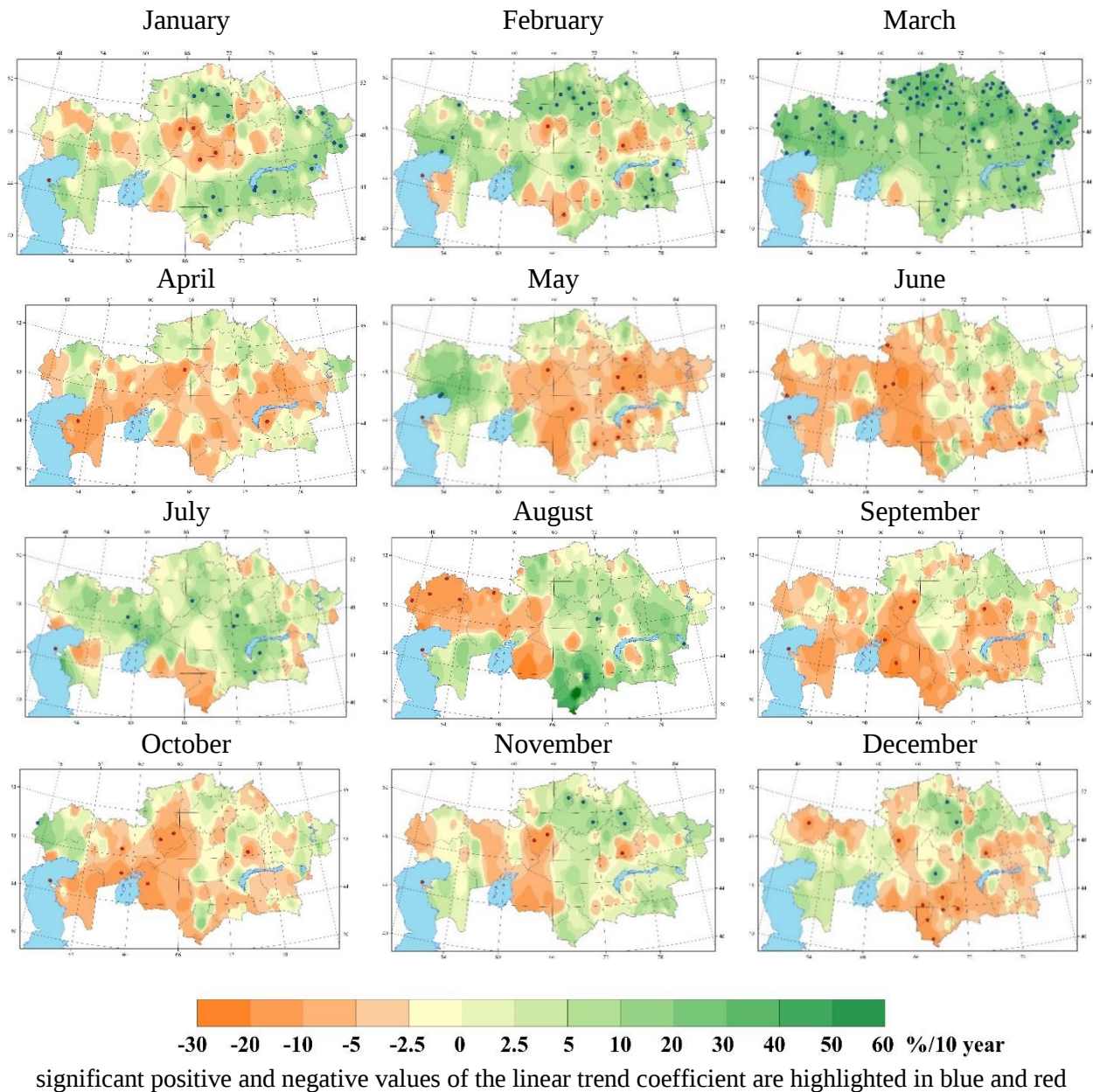
Figure 3.11 – Spatial distribution of values of the linear trend coefficient of monthly precipitation (%/10 years) calculated for the period 1976–2024
