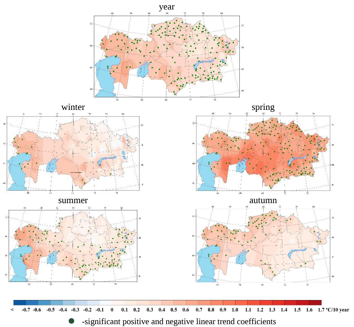
Figure 2.16 – Spatial distribution of values of the linear trend coefficient of mean annual and seasonal surface air temperature ( ^{\circ}\text{C}/10 years) calculated from observations for the period 1976–2024
