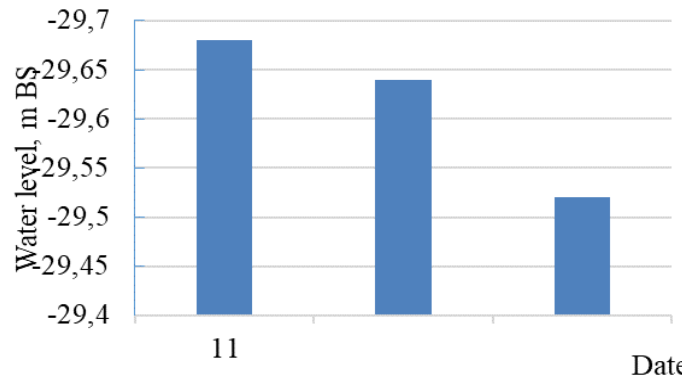
Figure. Graph of sea level changes in Saura on March 11, 2026.
