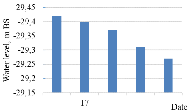
Figure. Graph of sea level changes in Fetisovo on March 16-17, 2026
