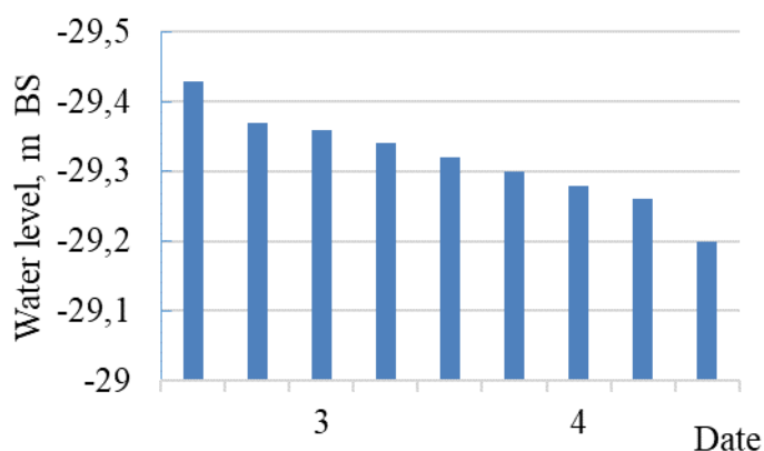
Figure. Graph of sea level changes in Fetisovo on March 02-04, 2026
