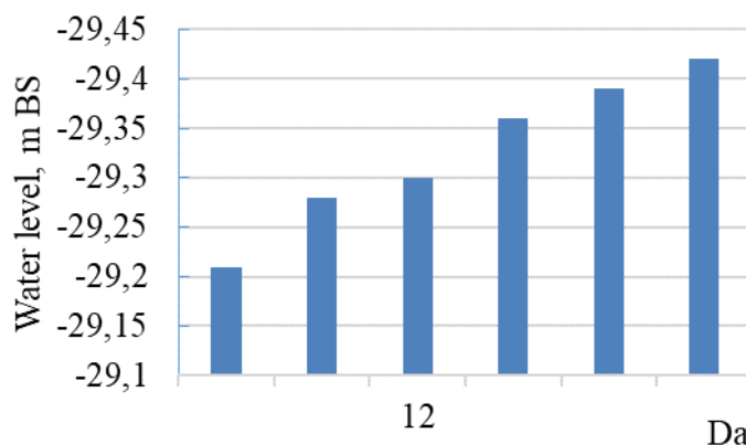
Figure. Graph of sea level changes in Fetisovo on March 11-12, 2026
