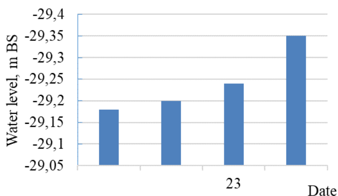
Figure. Graph of sea level changes in Fetisovo on March 22-23, 2026
