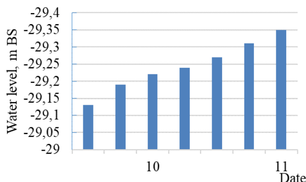
Figure. Graph of sea level changes in Fetisovo on March 09-11, 2026
