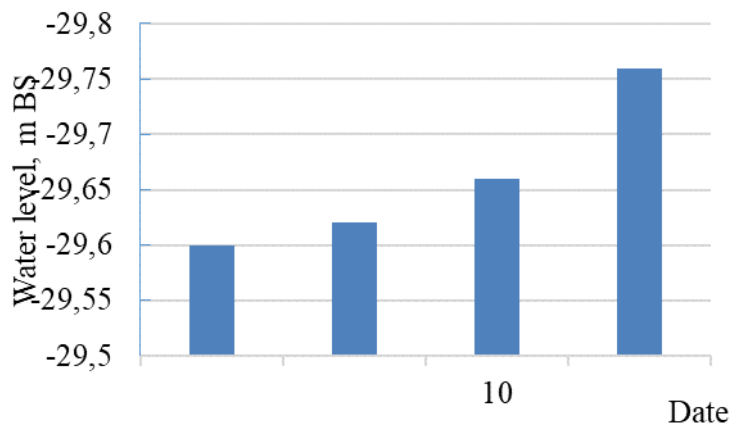
Figure. Graph of sea level changes in Fort-Shevchenko on March 09-10, 2026.
