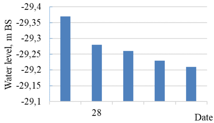
Figure. Graph of sea level changes in Fetisovo on March 27-28, 2026
