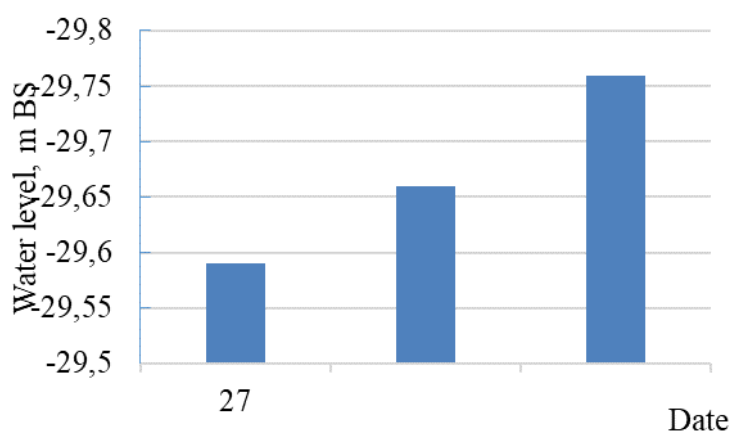
Figure. Graph of sea level changes in Fort-Shevchenko on March 27, 2026.
