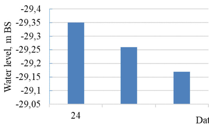
Figure. Graph of sea level changes in Fetisovo on March 24, 2026
