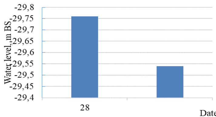
Figure. Graph of sea level changes in Saura on March 28, 2026.
