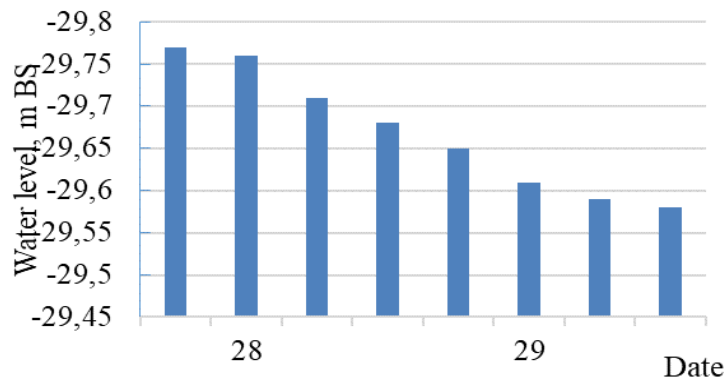
Figure. Graph of sea level changes in Aktau on March 27-29, 2026.
