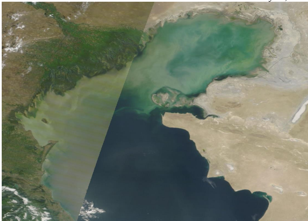
Fig.1 Space image of the Caspian Sea, July 29, 2026 (NASA/GSFC)
