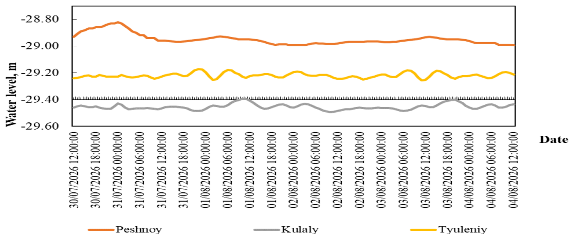
Fig .3 Forecast of sea level in the points of the North Caspian
