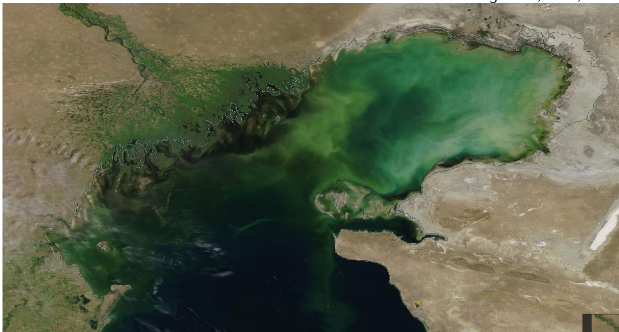
Fig.1 Space image of the Caspian Sea, August 04, 2026 (NASA/GSFC)
