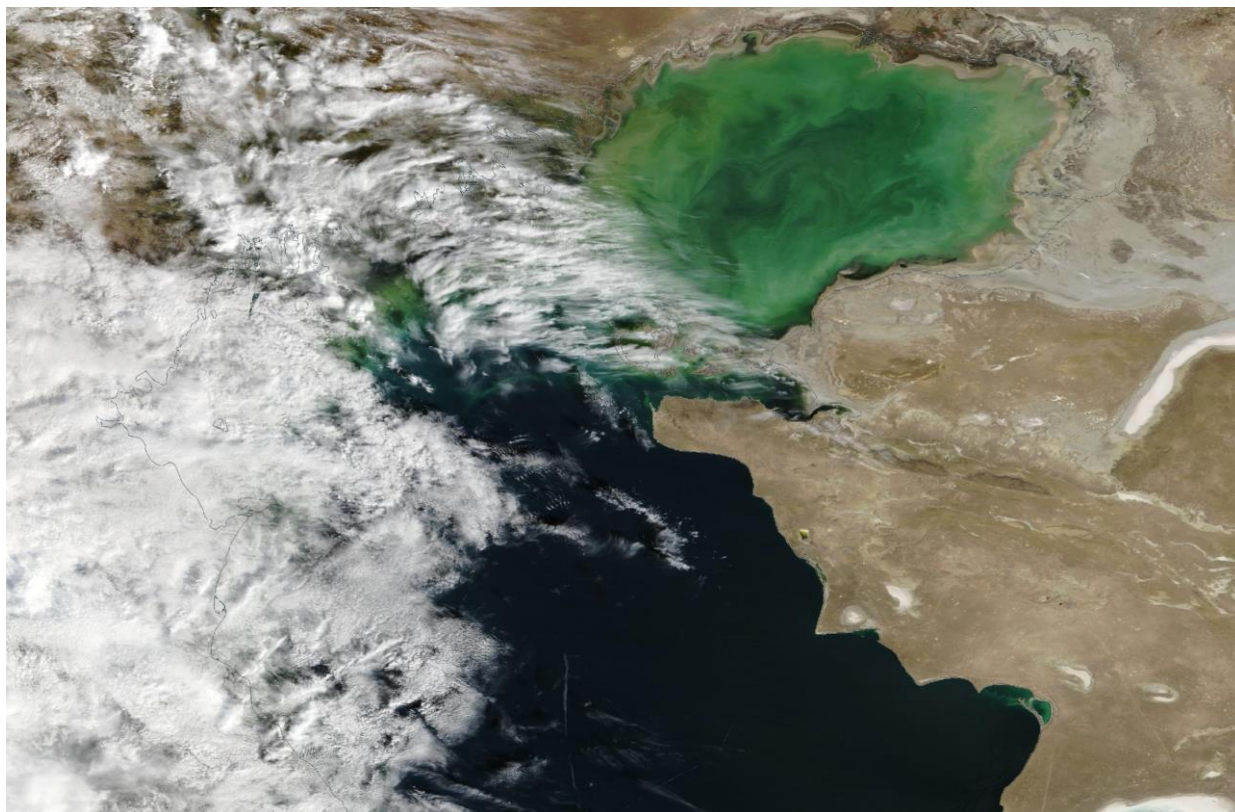
Fig.1 Space image of the Caspian Sea, October 1, 2026 (NASA/GSFC)
