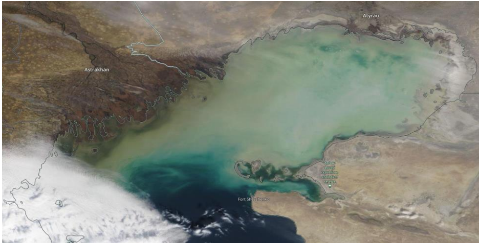
Fig 1. Ice conditions on the Caspian Sea, 03 March, 2022. Image of the «MODIS Project at NASA Aqua»
