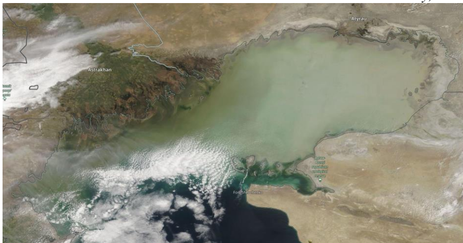
Fig.1 Space images of the Caspian Sea, 01 May, 2022, NAGA/GSFC
