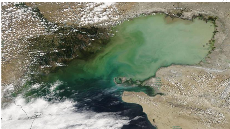
Fig.1 Space images of the Caspian Sea, 17 May, 2022, NAGA/GSFC
