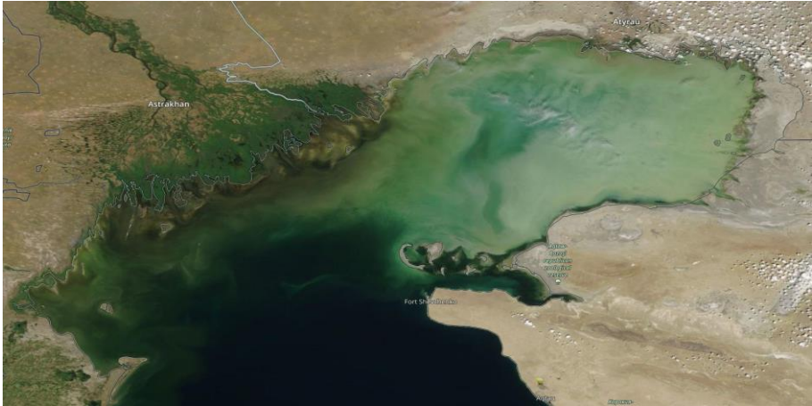
Fig.1 Space images of the Caspian Sea, 20 June, 2022, NAGA/GSFC
