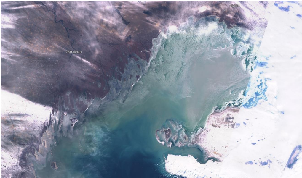
Space image of the Caspian Sea, December 15, 2024 (Sentinel-3 OLCI)
