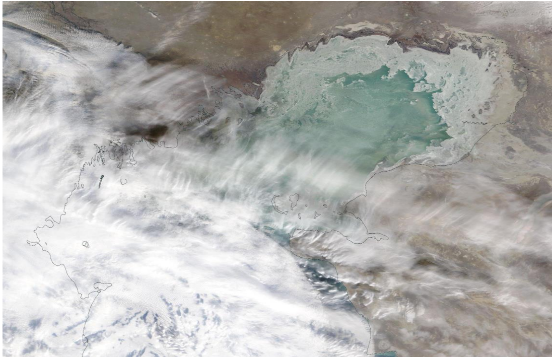
Space image of the Caspian Sea, December 27, 2024 (NASA/GSFC)
