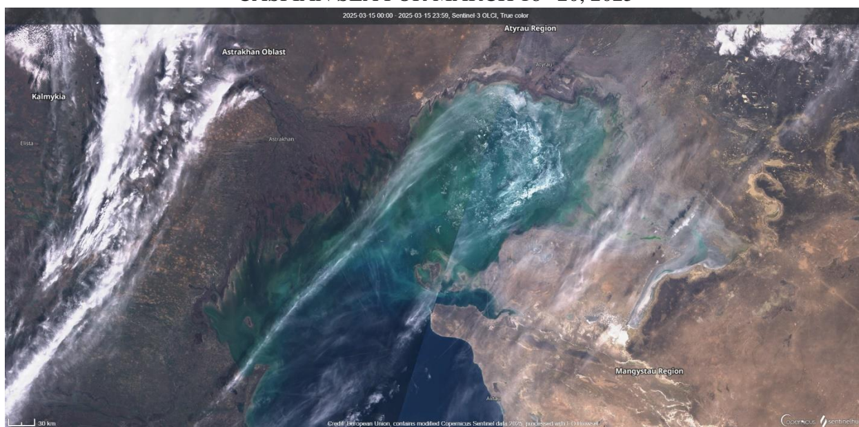
Fig.1 Space image of the Caspian Sea, March 15, 2025 (NASA World View)
