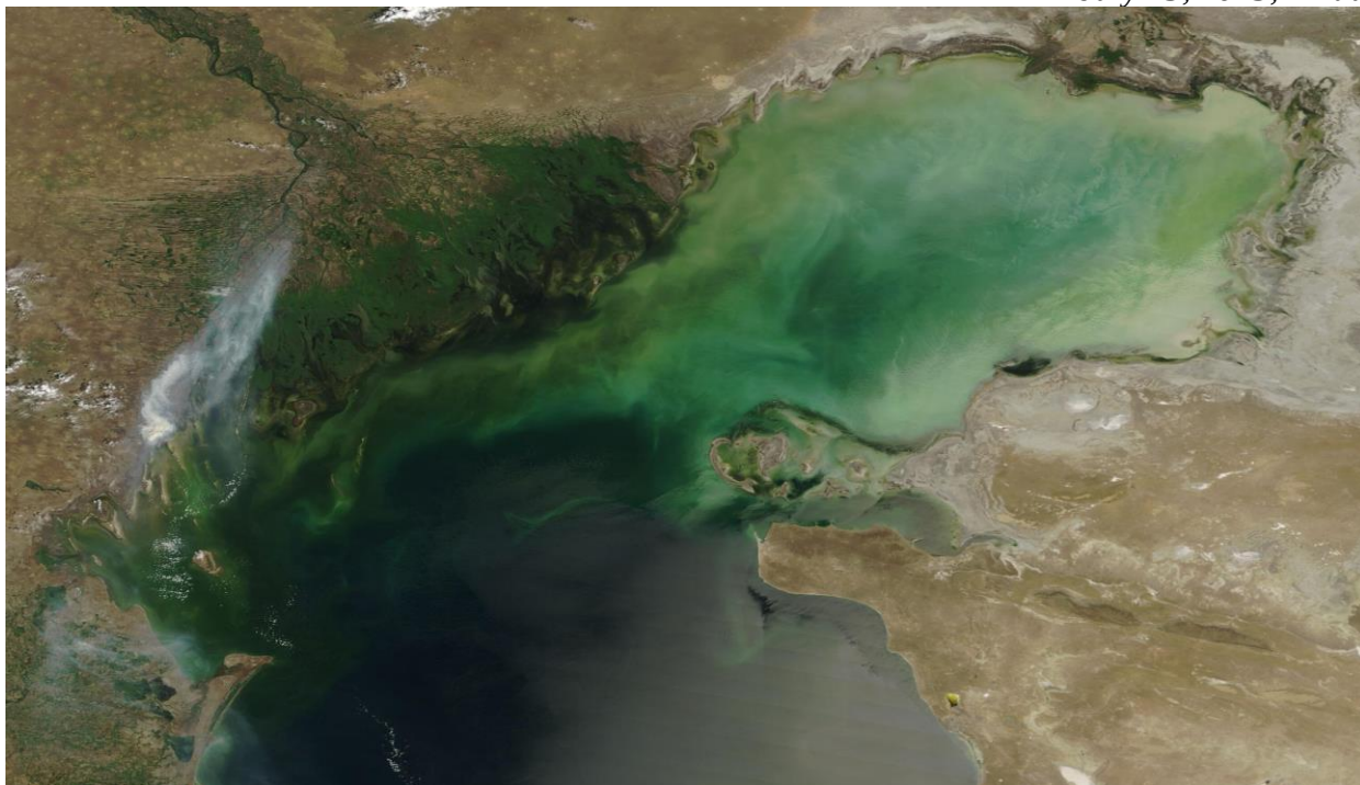
Fig.1 Space image of the Caspian Sea, July 23, 2025 (NASA/GSFC)
