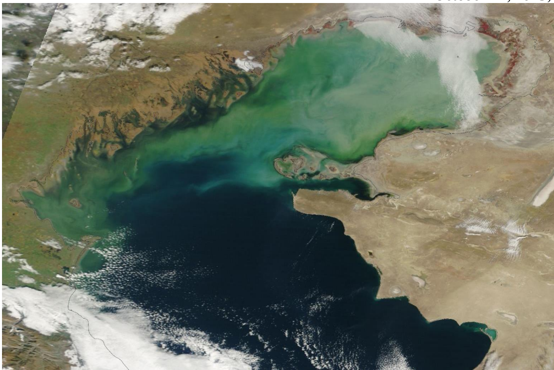
Fig.1 Space image of the Caspian Sea, October 22, 2025 (NASA/GSFC)
