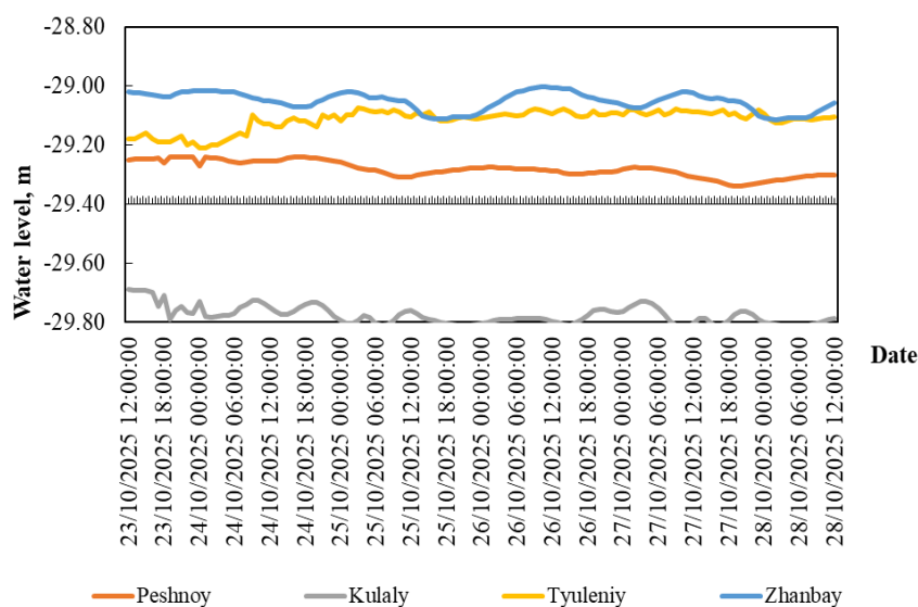
Fig .3 Forecast of sea level in the points of the North Caspian
