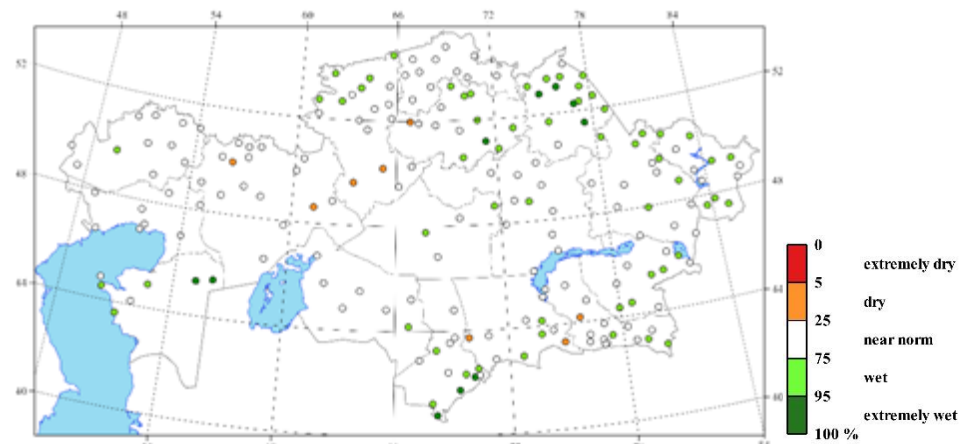
Figure 4 – Spatial distribution of probability of non-exceedance of precipitation in December 2025. Probabilities are calculated from data of the period 1941–2025
